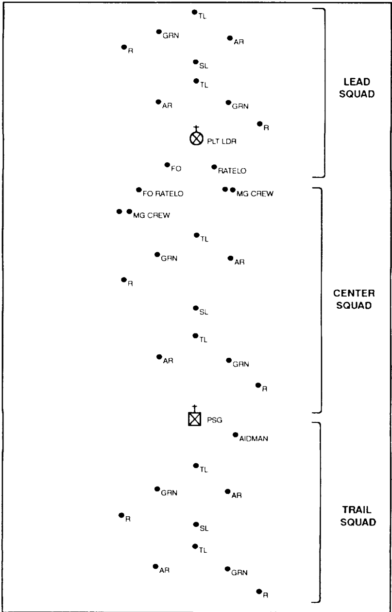
Figure 2-11. Platoon column.
